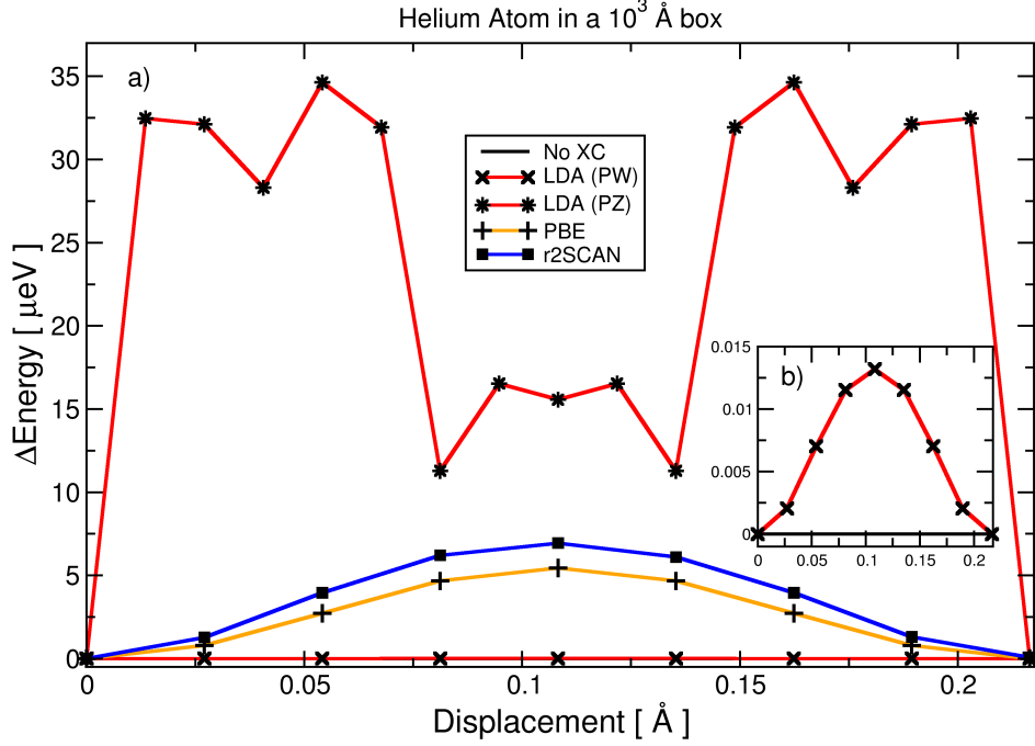
Figure 5.2: Change in the total energy of an isolated Helium atom as the atom is displaced along the (111) direction of a (10 \text{\AA})^3 cubic unit cell. A 80^3 FFT grid to represent the density and a single k-point at the Gamma point was used for Brillouin zone integration. Sub-figure b ) is the same plot with the y-axis scaled to allow the LDA (PW) [3] result to be seen.
