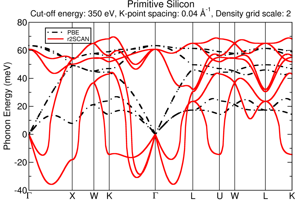
Figure 5.4: Phonon spectra calculated for a silicon primitive cell using the PBE and r2SCAN functionals. Calculated via finite displacement using the non-diagonal supercell method, equivalent to a 3 \times 3 \times 3 q-point sampling grid.
