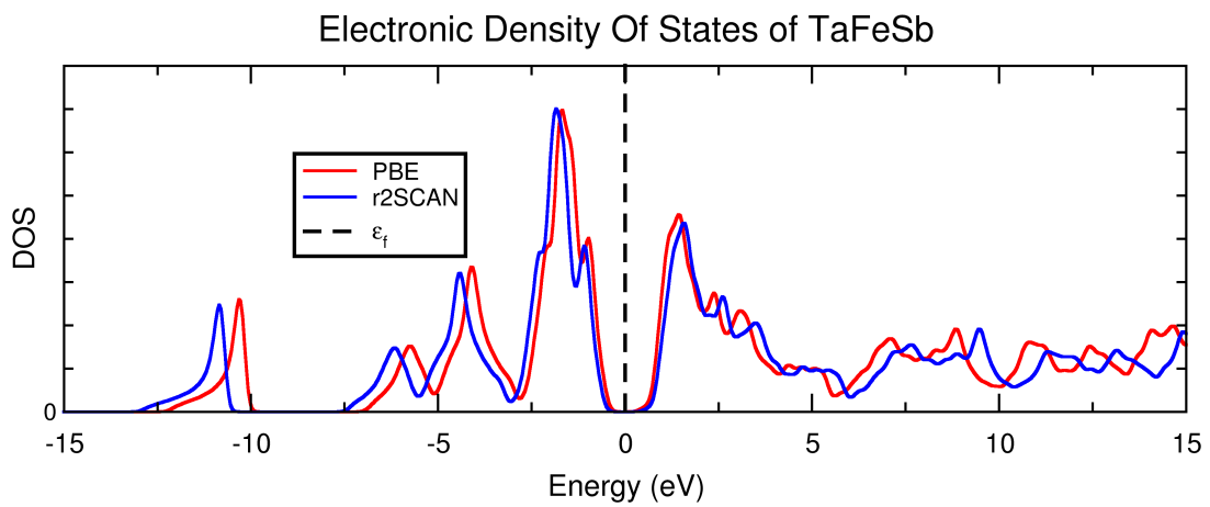
Figure 1.3: Electronic density of states (DOS) of TaFeSb computed using DFT with a GGA functional (PBE) and a mGGA functional (r2SCAN), where the energies of both calculations have been shifted so that the Fermi level is at 0 eV.
